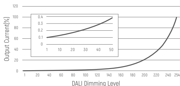
DALI Curve
