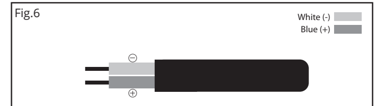
All the Linear High Bay products are fitted with a dimming cable. IF the luminaire is not to be fitted to a dimming system ensure that the ends of the dimming cable and securely terminated and isolated from any electrical interference
