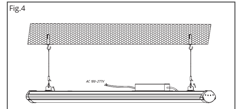
When the product is securely mounted on the suspension point make the cable connections for mains power and dimming
